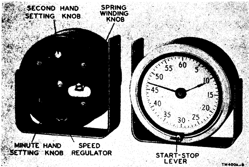
Figure 8. Timer PH-29, controls.
